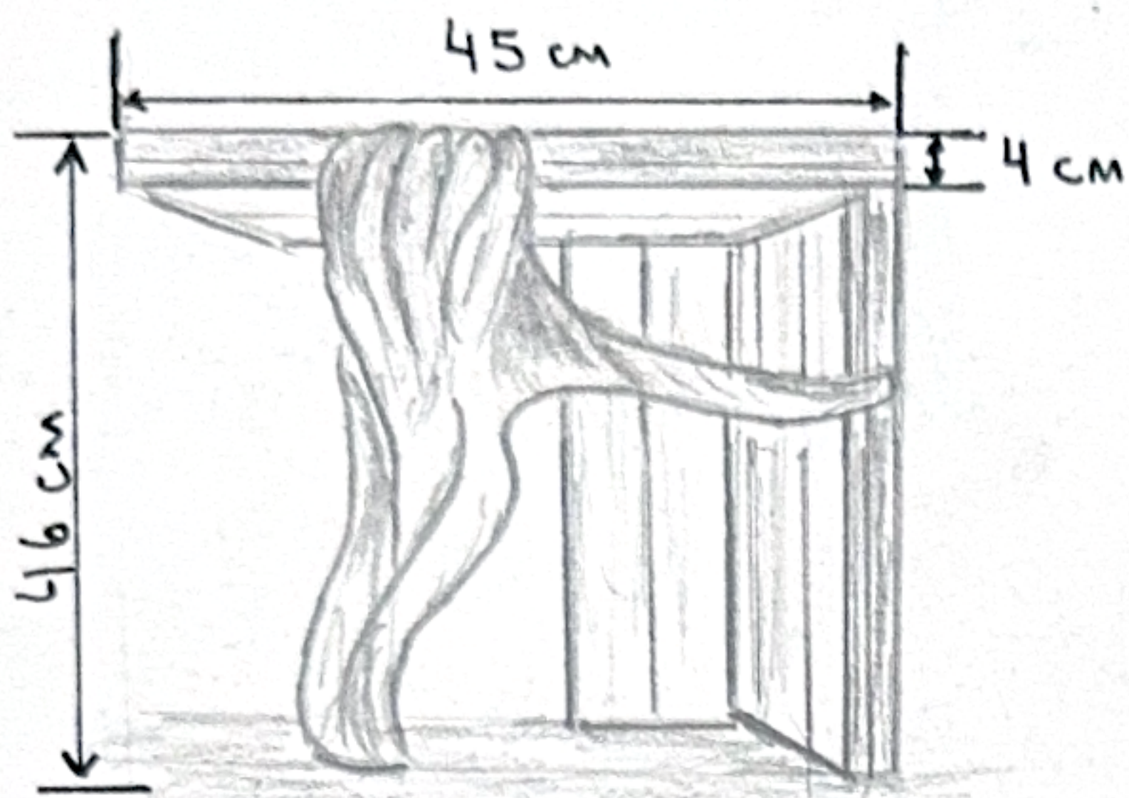
VISTA FRONTAL
